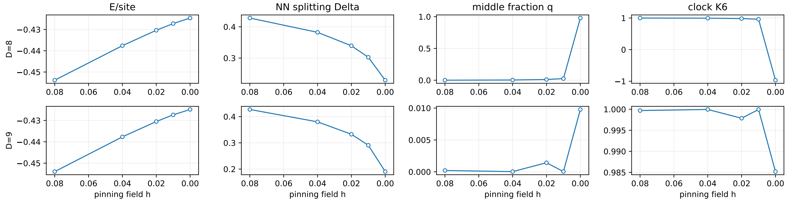
Izar replica 1, J_2=0.30 , plaquette source: available optimization endpoints versus h
