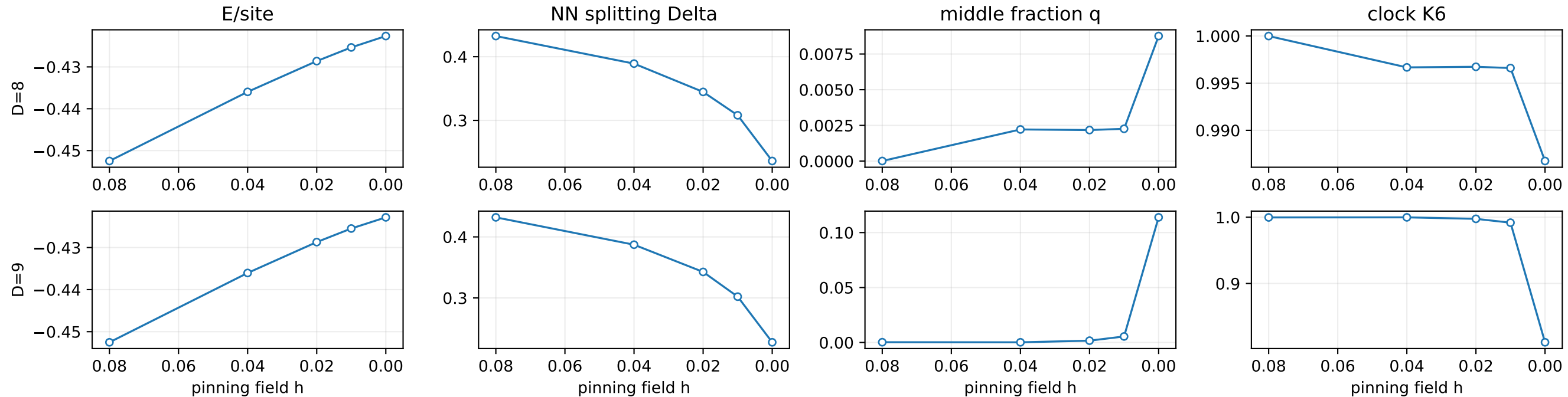
Izar replica 1, J_2=0.31 , plaquette source: available optimization endpoints versus h
