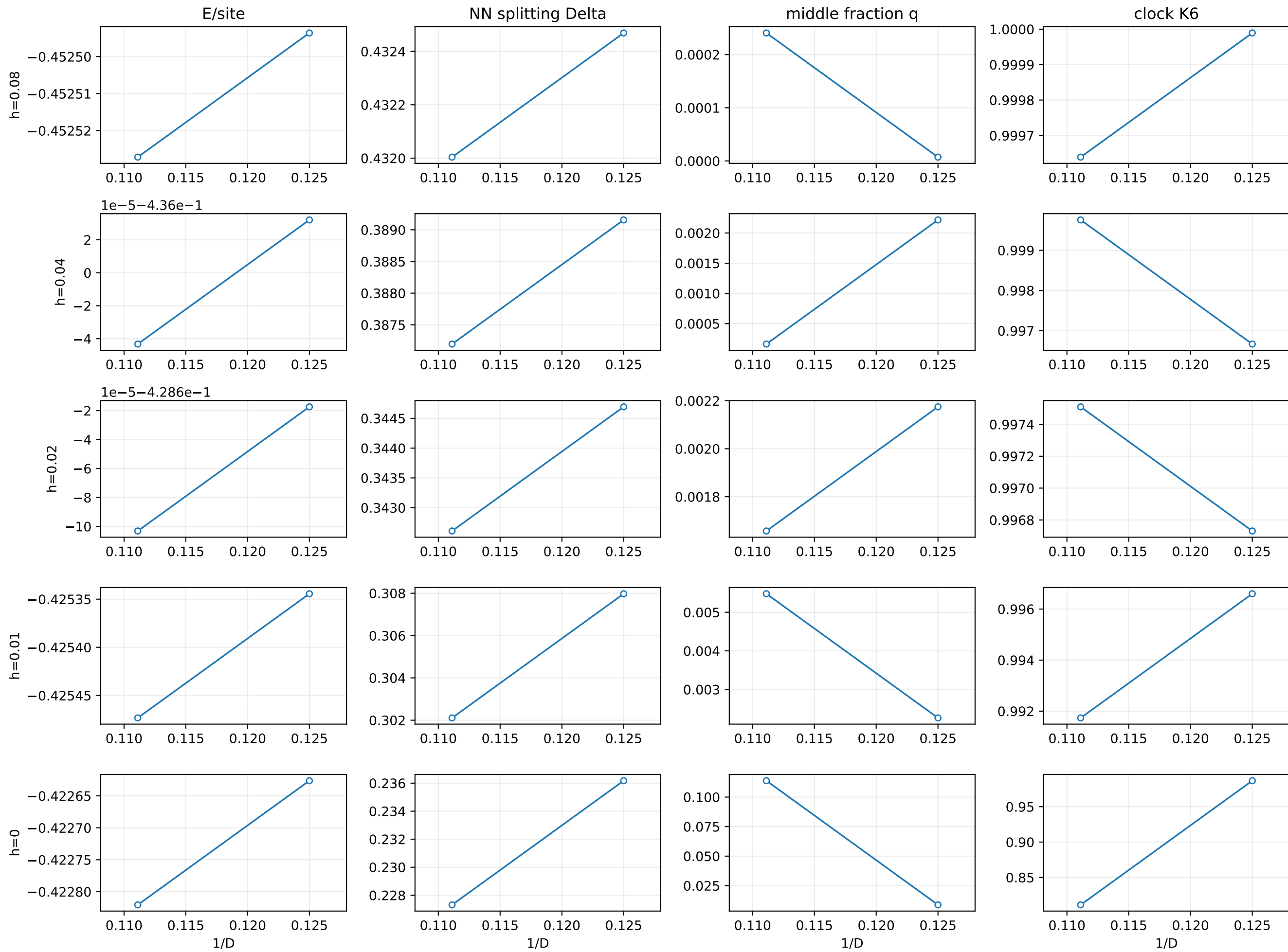
Izar replica 1, J2=0.31, plaquette source: fixed-h trends; only h=0 energy is unbiased
