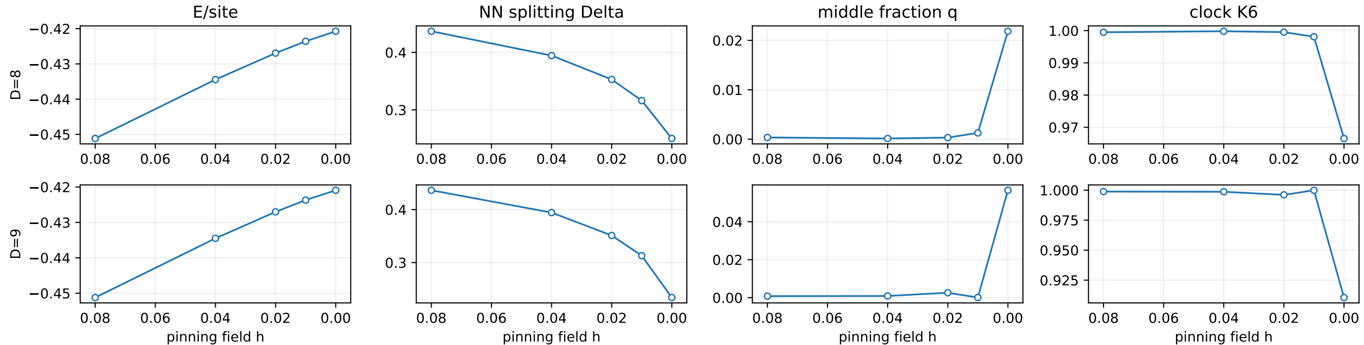
Izar replica 1, J_2=0.32 , plaquette source: available optimization endpoints versus h
