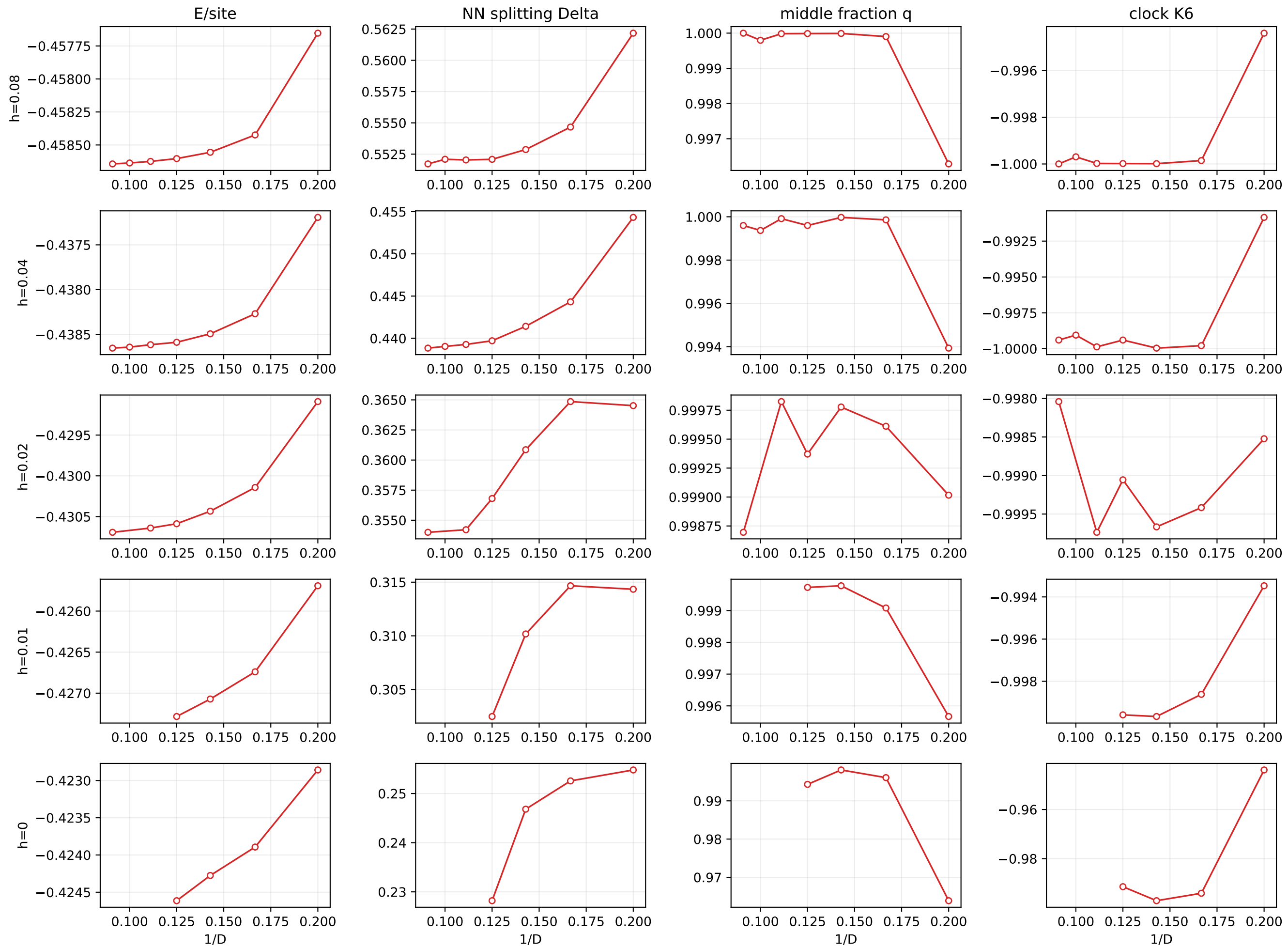
Kuma replica 1, J2=0.30, dimer source: fixed-h trends; only h=0 energy is unbiased
