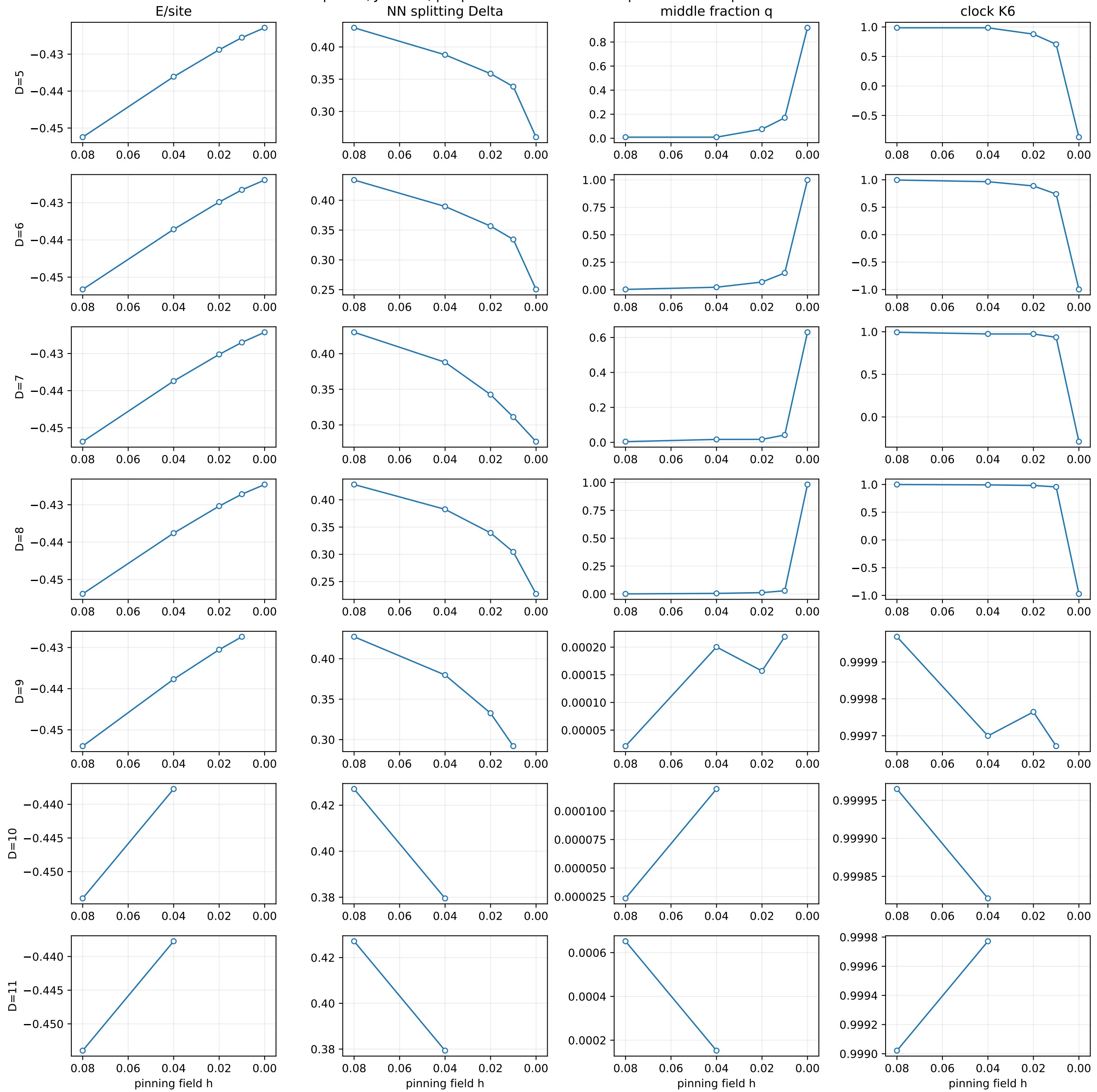
Kuma replica 1, J2=0.30, plaquette source: available optimization endpoints versus h
