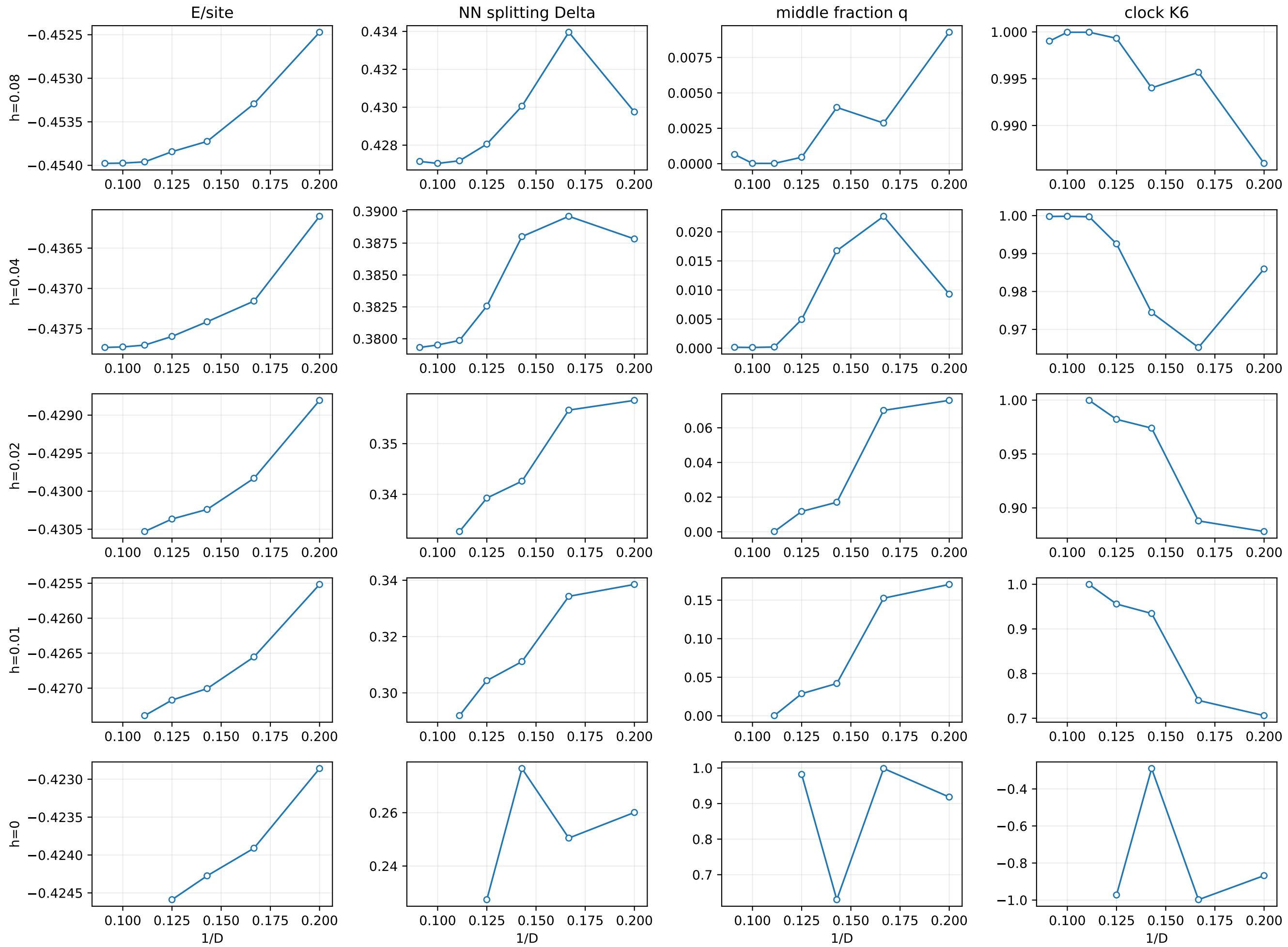
Kuma replica 1, J_2=0.30 , plaquette source: fixed-h trends; only h=0 energy is unbiased
