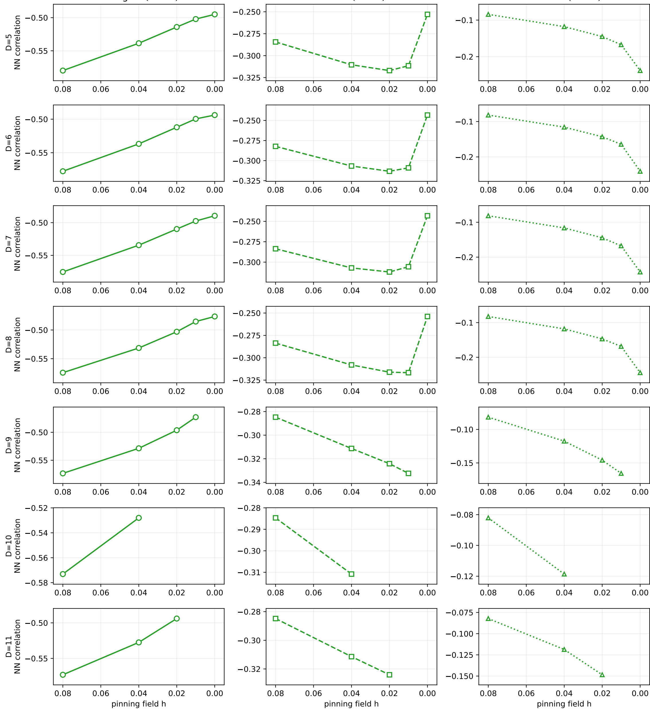
Kuma replica 1, J_2=0.30 , rank-split source: one rank per panel (independent vertical scales) strongest (rank1) middle (rank2) weakest (rank3)
