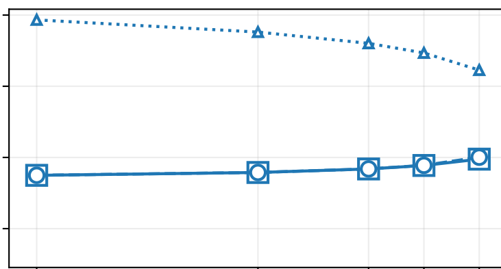
Plaquette pin
