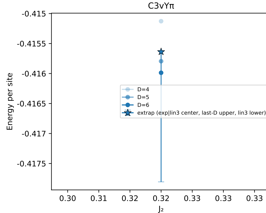
Energy per site vs J_2 — combined
