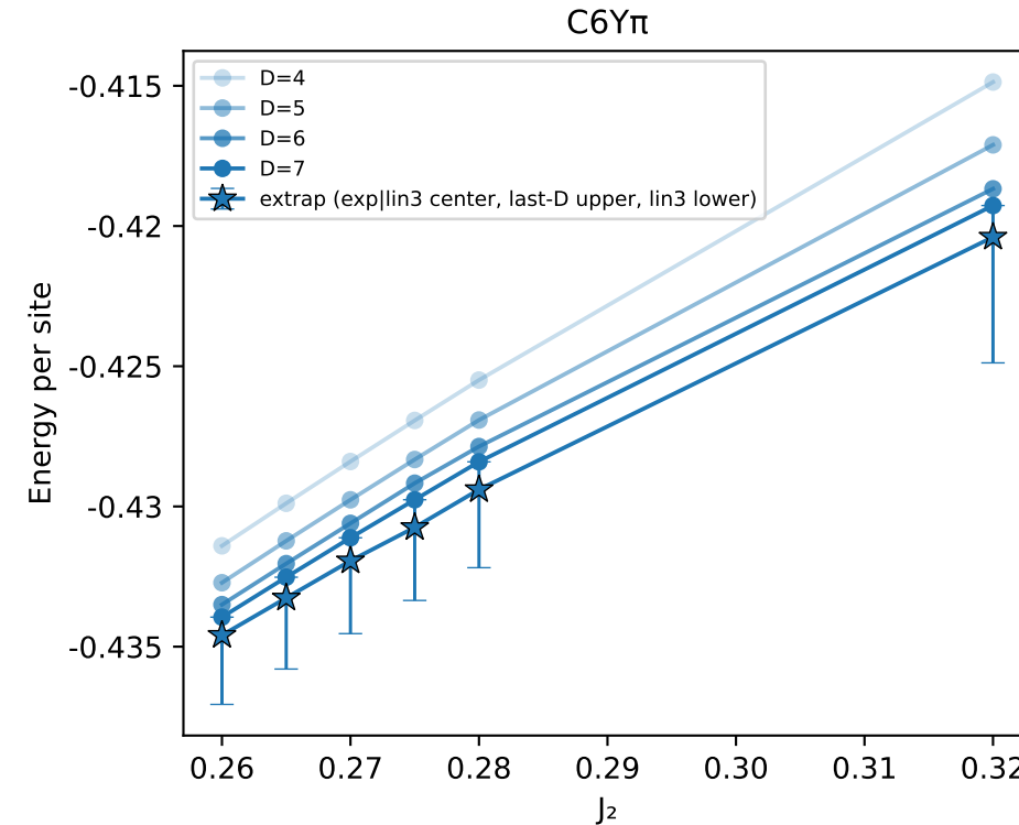
Energy per site vs J_2 — combined
