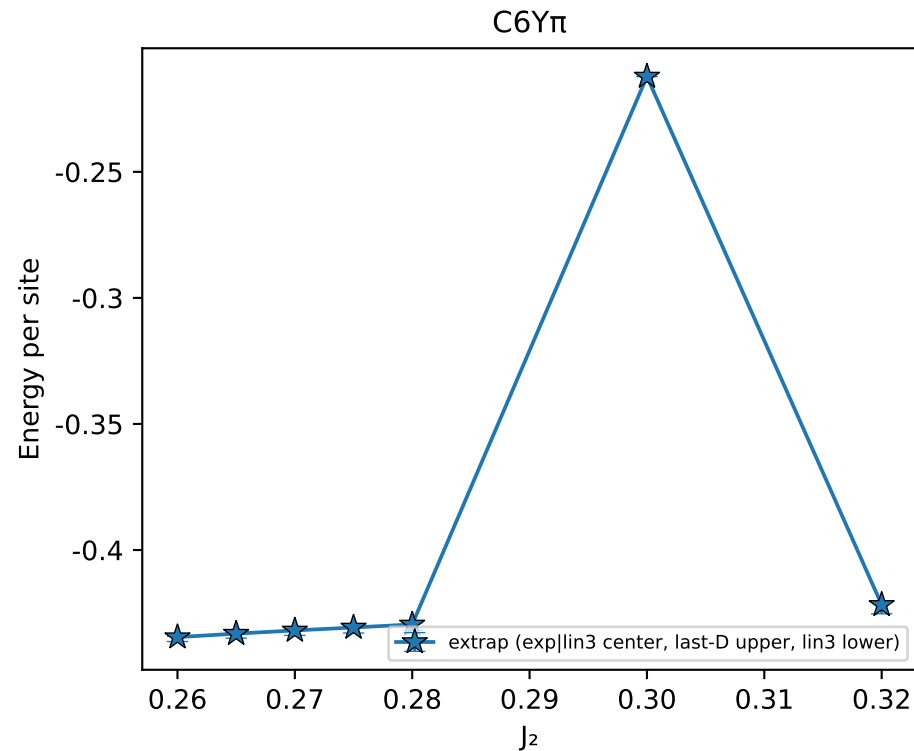
Energy per site vs J_2 — extrapolated
