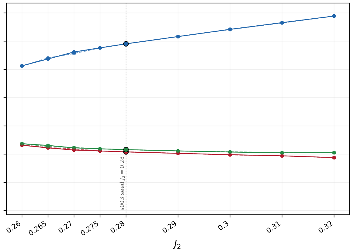
Plaquette seed, D = 8
