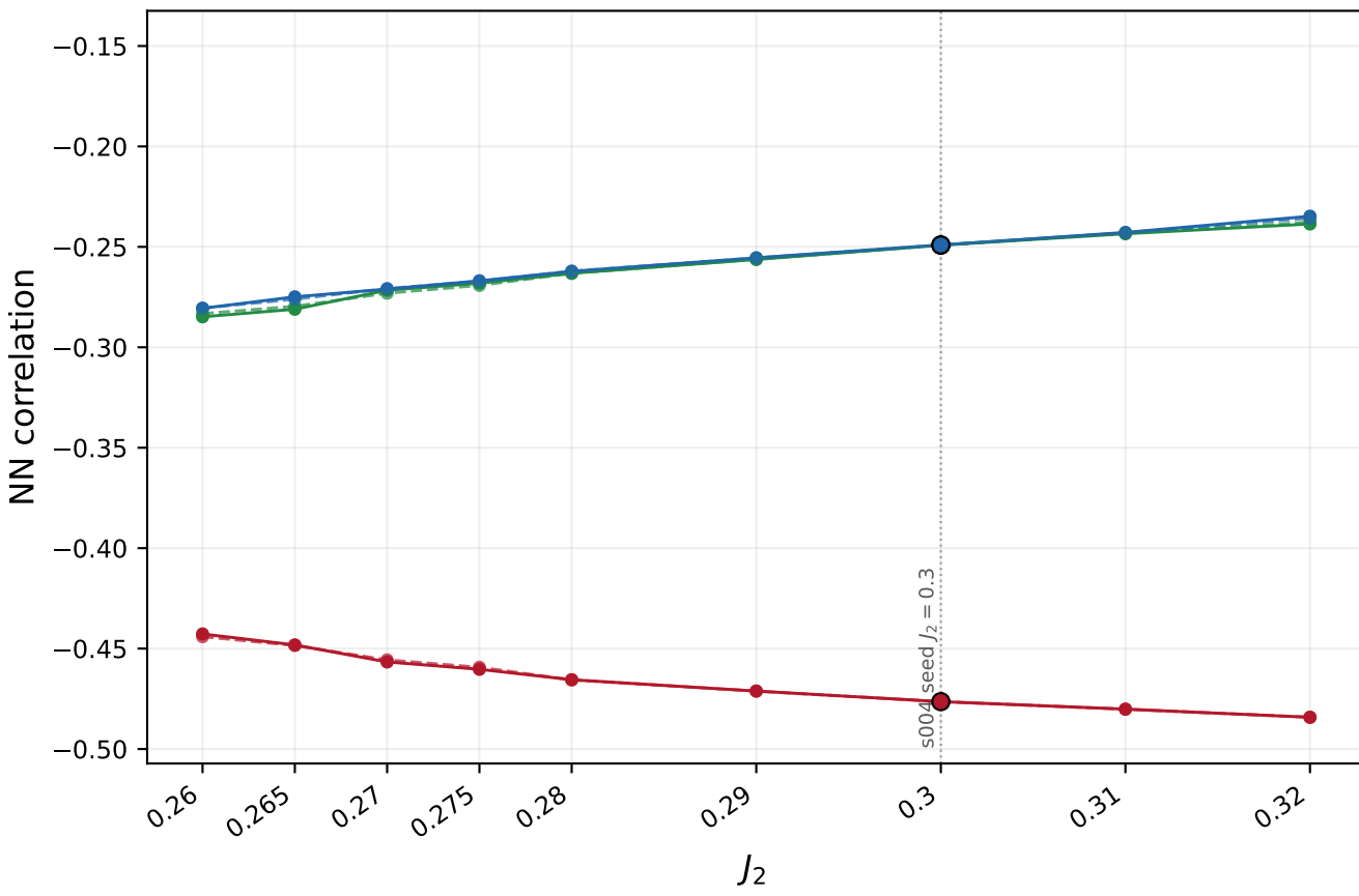
Dimer-plaquette seed, D = 8
