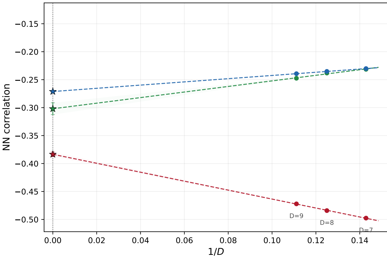
Dimer-plaquette seed, J_2 = 0.32
