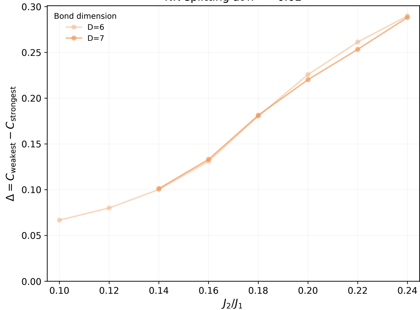
NN splitting at h = -0.02
