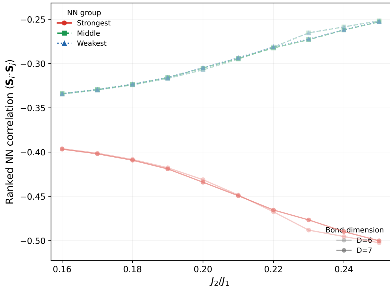
NN correlations at h = -0.01
