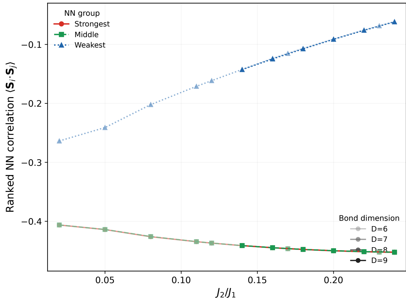
NN correlations at h = +0.08
