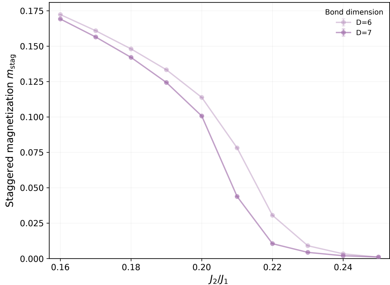
Staggered magnetization at h = +0.01
