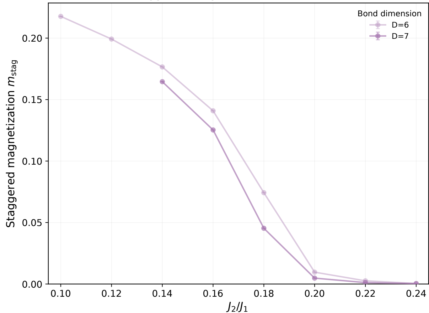
Staggered magnetization at h = +0.02
