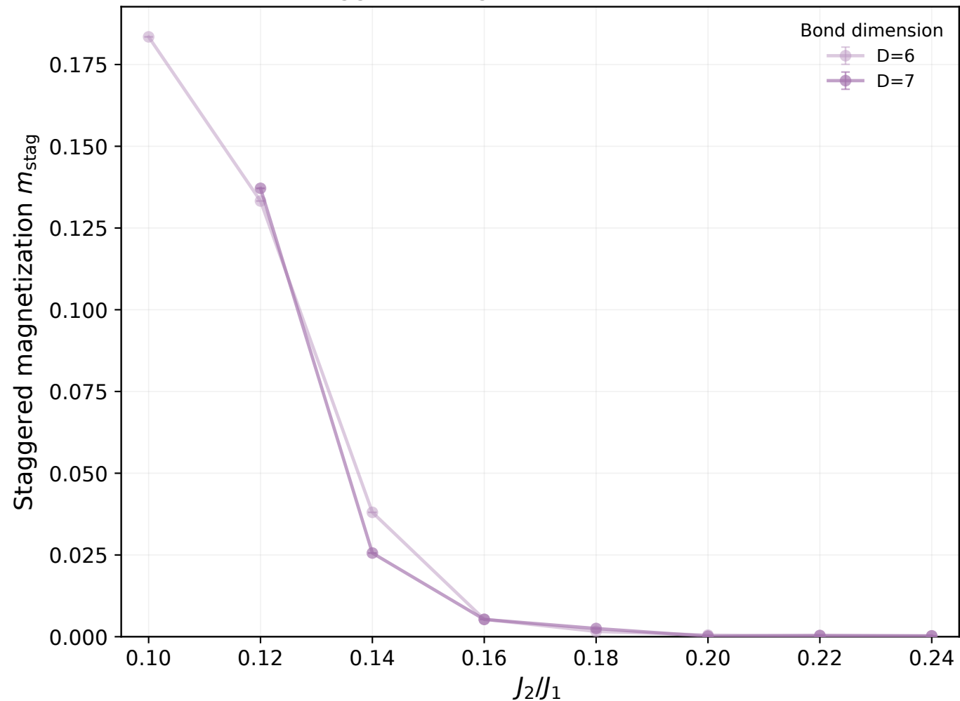
Staggered magnetization at h = +0.04
