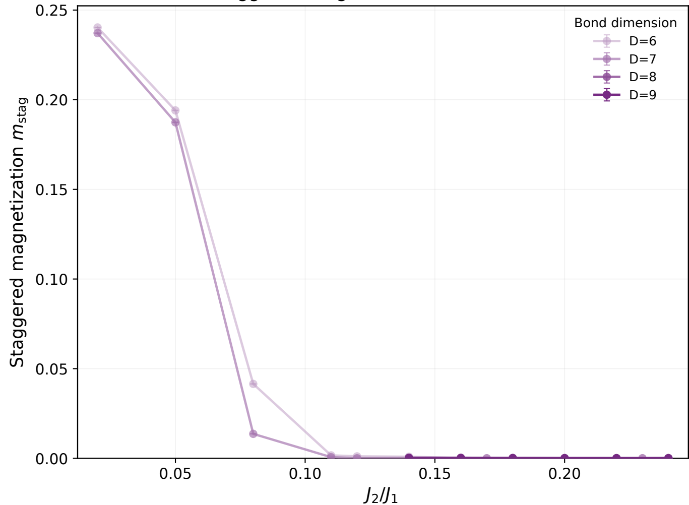
Staggered magnetization at h = +0.08
