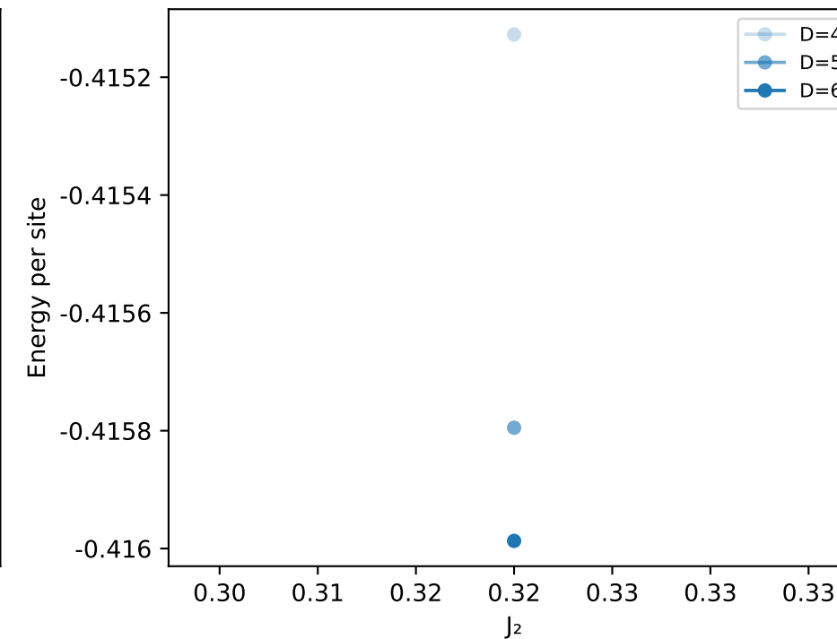
C3vY \pi
