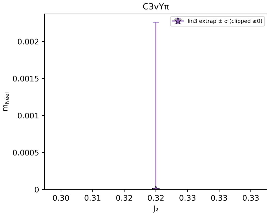
m_{\text{Néel}} vs J_2 — lin3 extrapolated \pm \sigma
