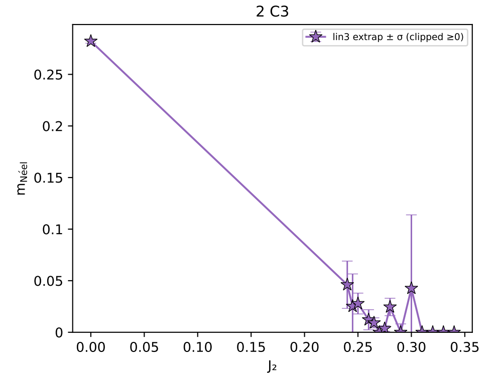
m_{\text{Néel}} vs J_2 — extrapolated \pm \sigma
