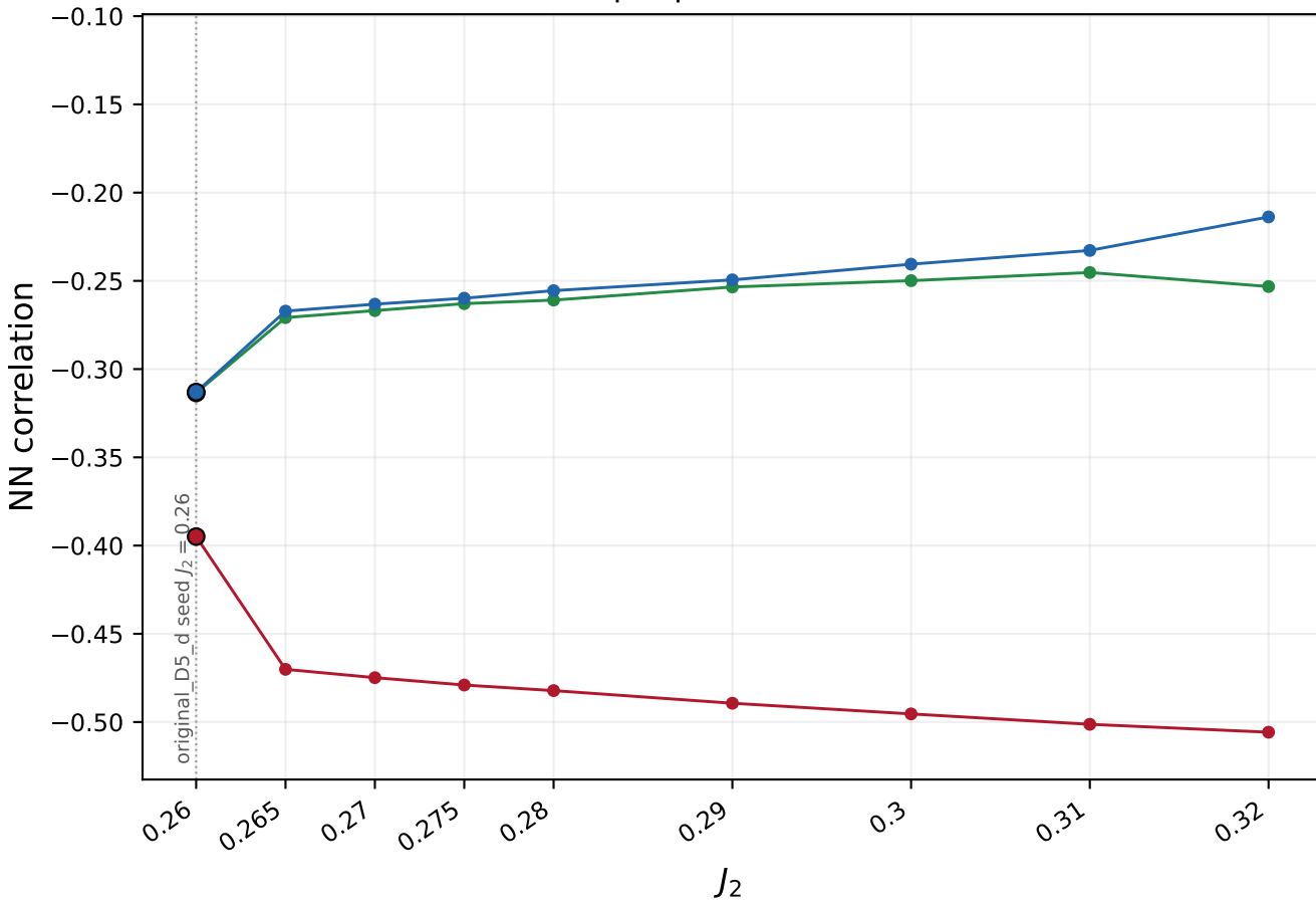
Dimer-plaquette seed, D = 5
