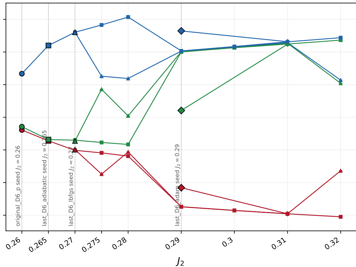
Plaquette seed, D = 6
