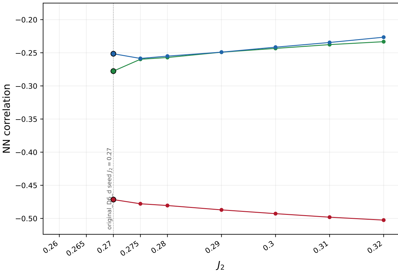
Dimer-plaquette seed, D = 6
