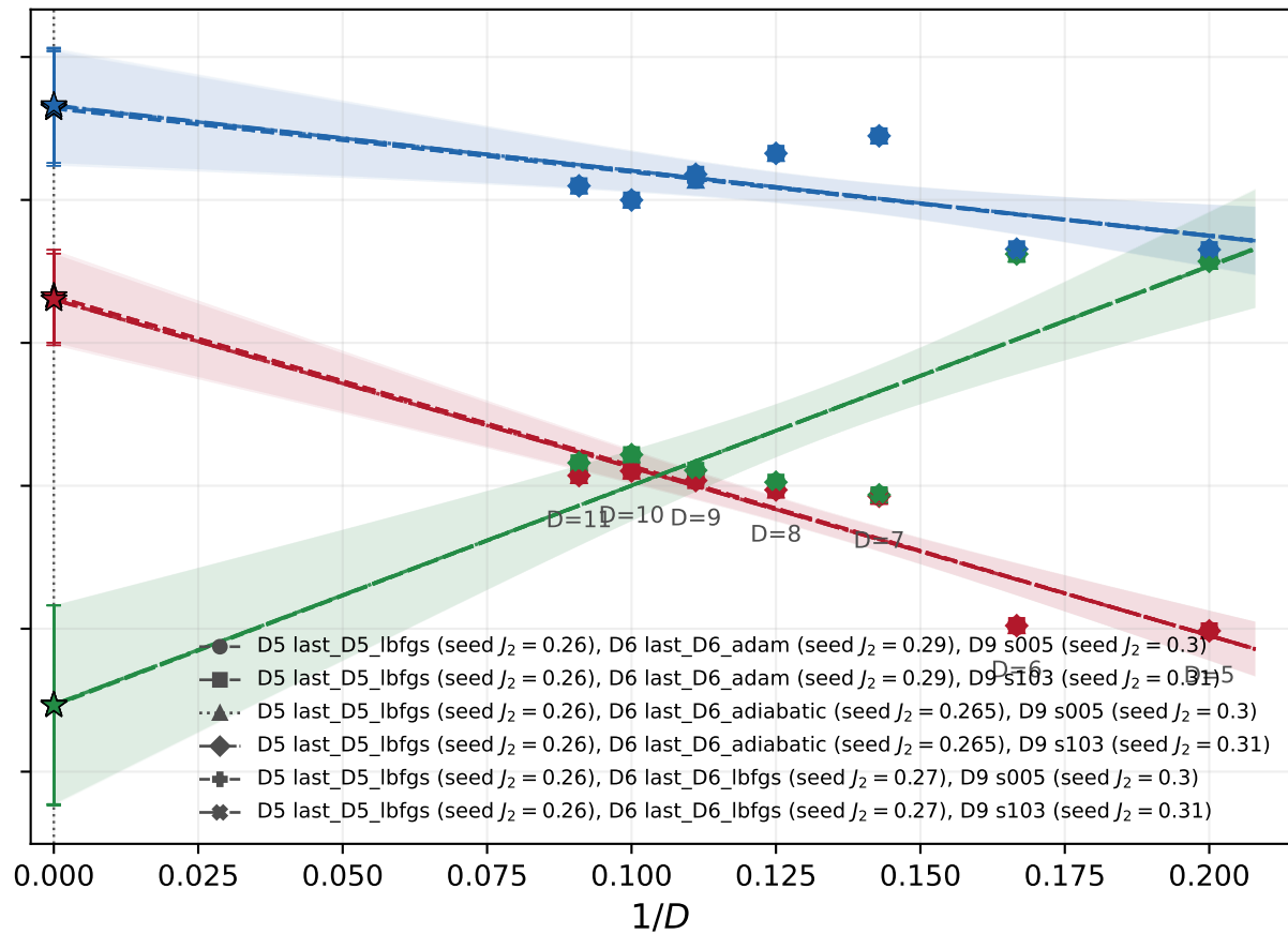
Plaquette seed, J_2 = 0.31
