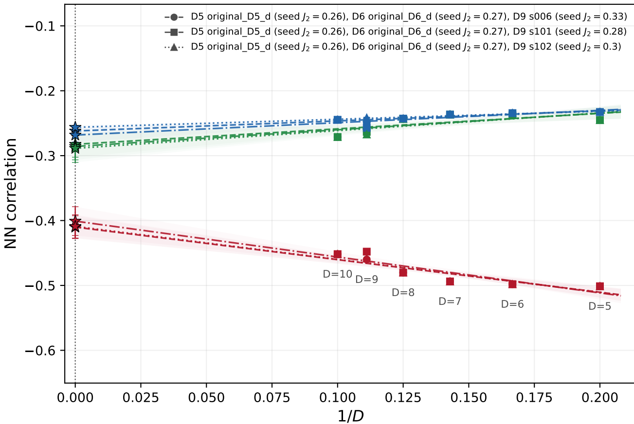
Dimer-plaquette seed, J_2 = 0.31
