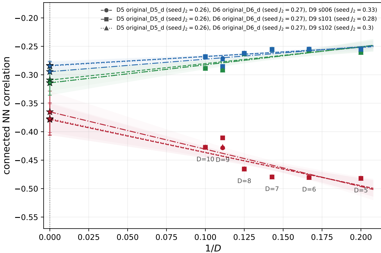
Dimer-plaquette seed, J_2 = 0.28
