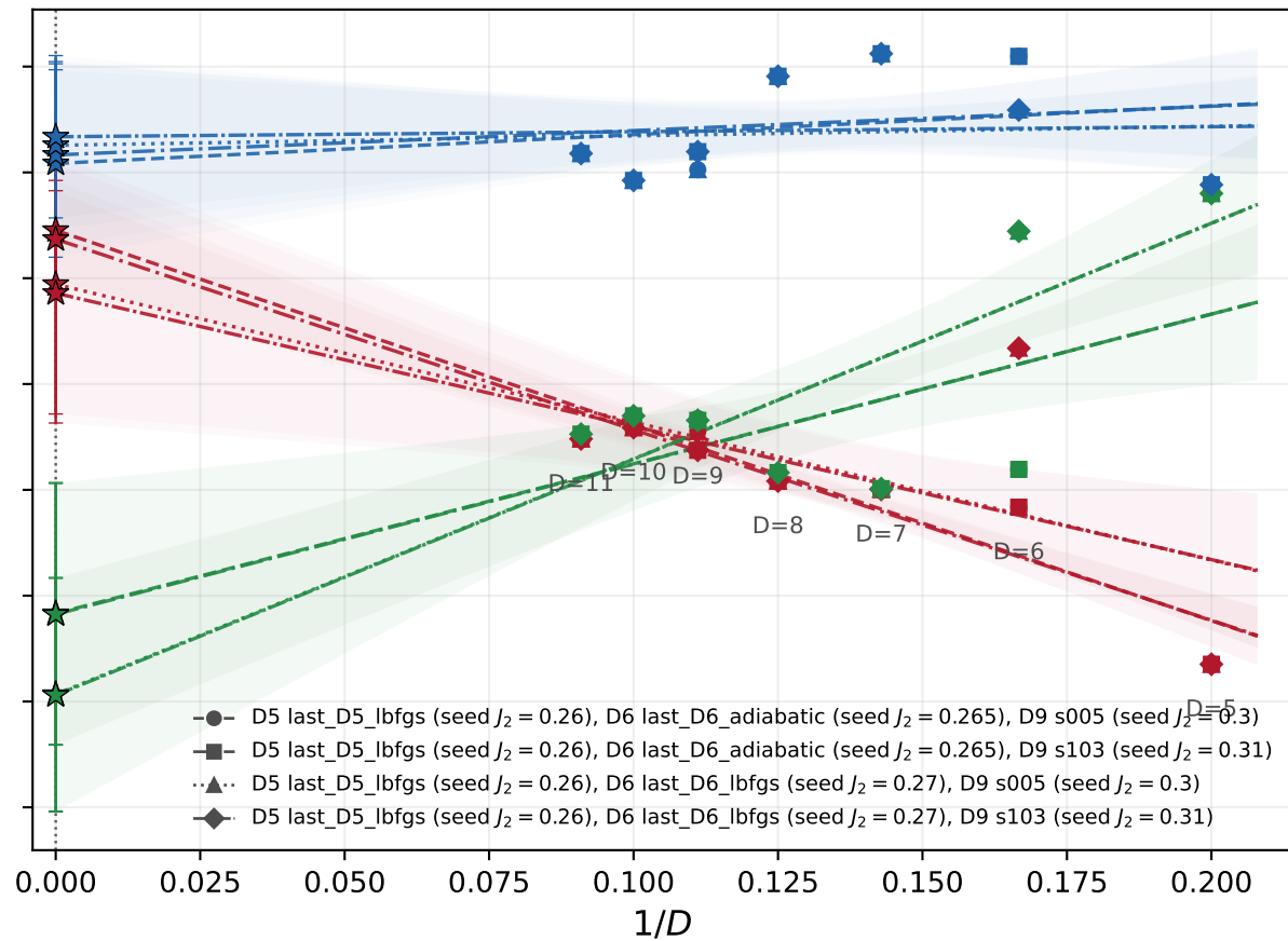
Plaquette seed, J_2 = 0.28
