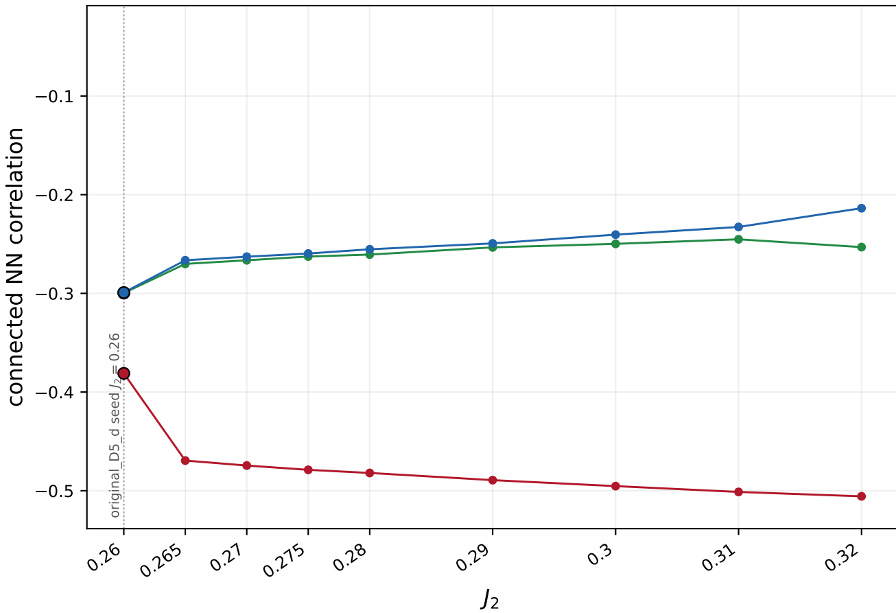
Dimer-plaquette seed, D = 5
