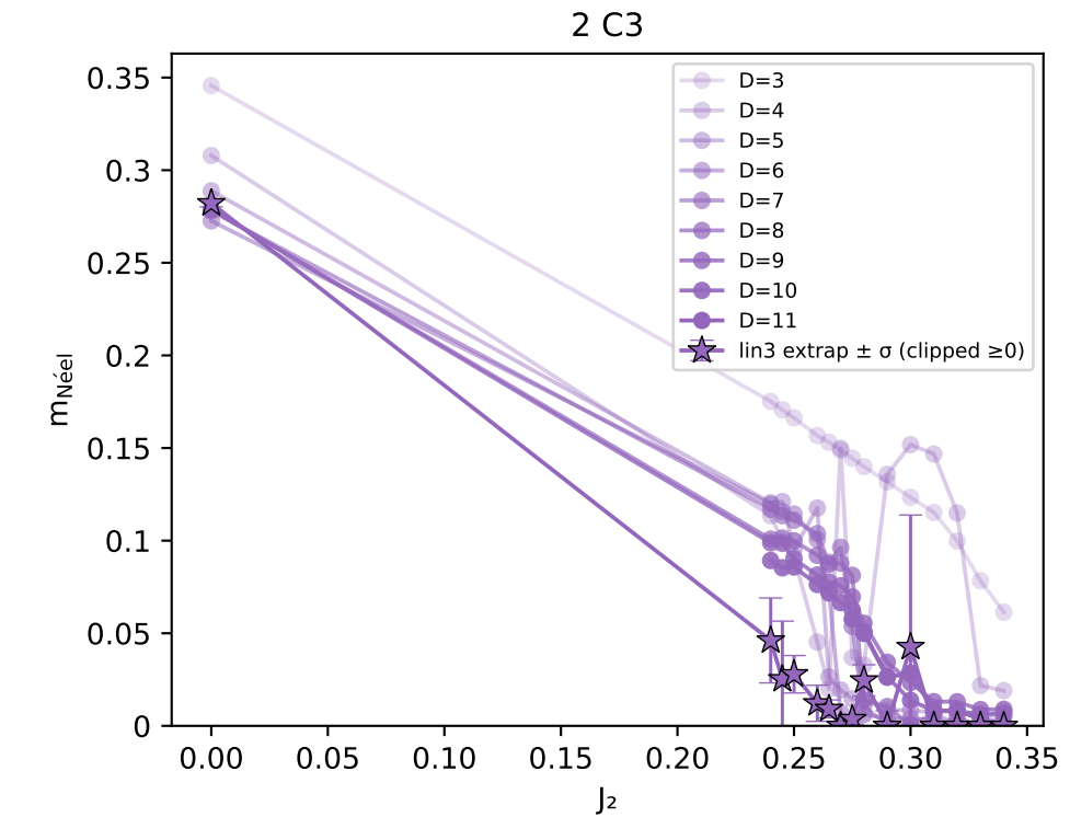
m_{\text{Néel}} vs J_2 — combined
