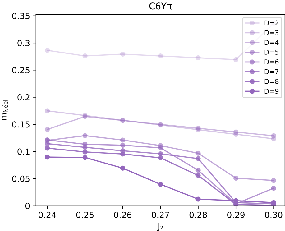
m Néel vs J 2 — raw D curves
