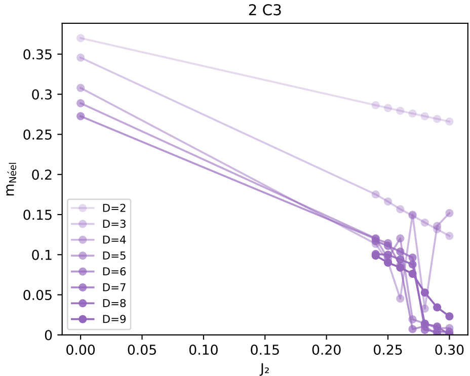
m Néel vs J 2 — raw D curves
