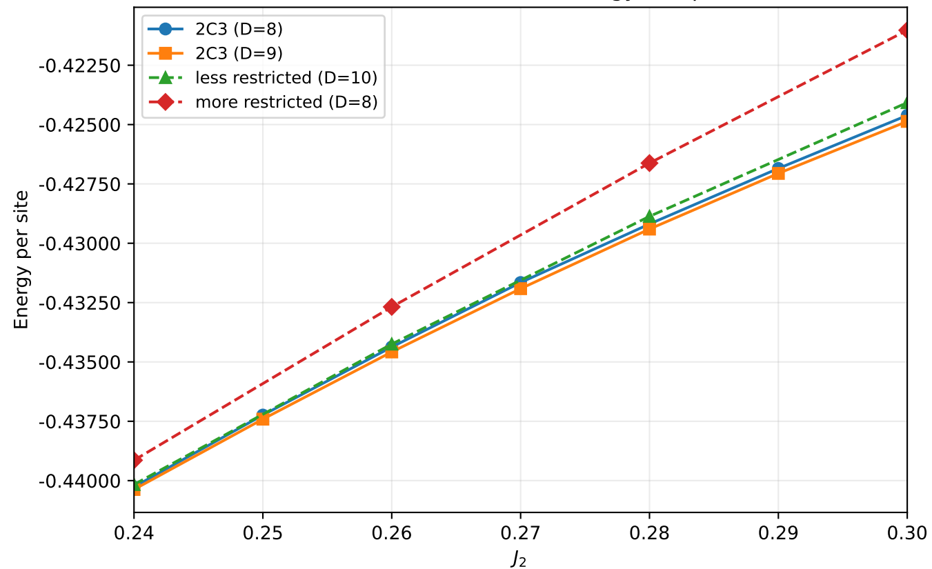
2C3 and restricted-ansatz energy comparison
