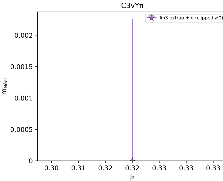
m_{\text{Néel}} vs J_2 — lin3 extrapolated \pm \sigma
