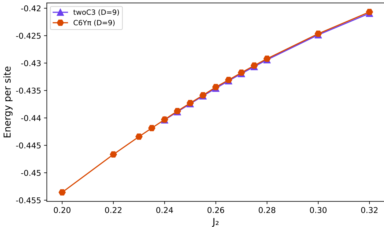
Energy: twoC3 (D=9) vs C6Y \pi (D=9)
