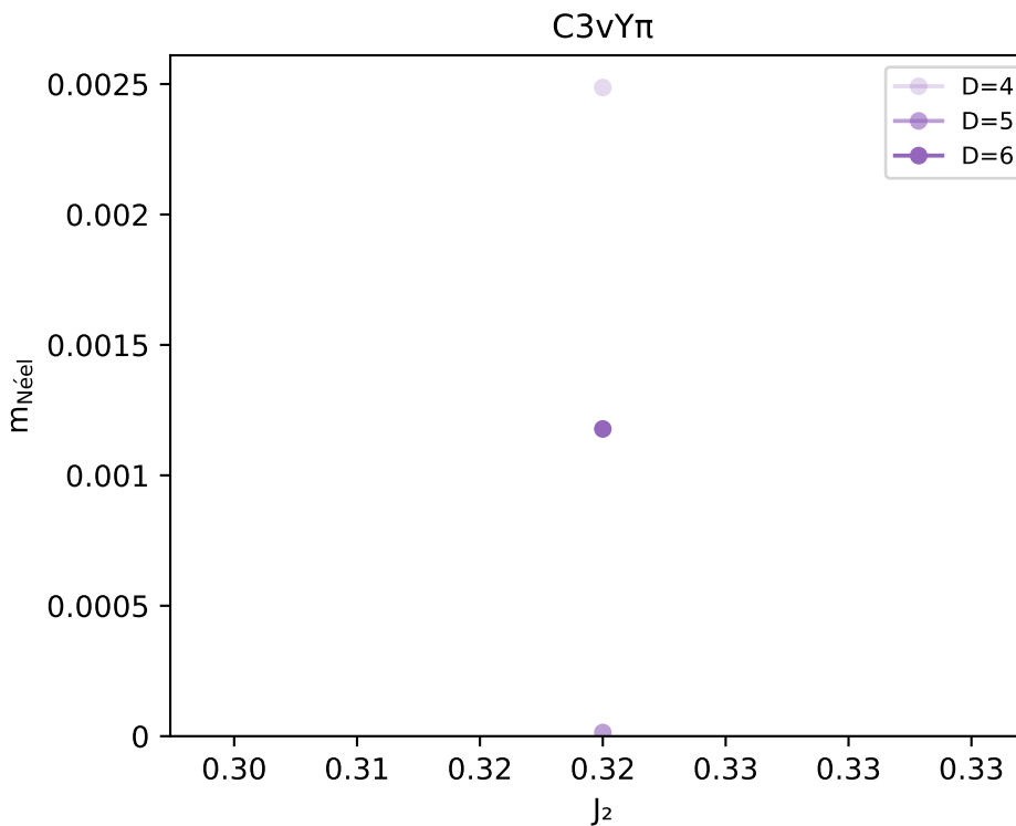
m_{\text{Néel}} vs J_2 — raw D curves
