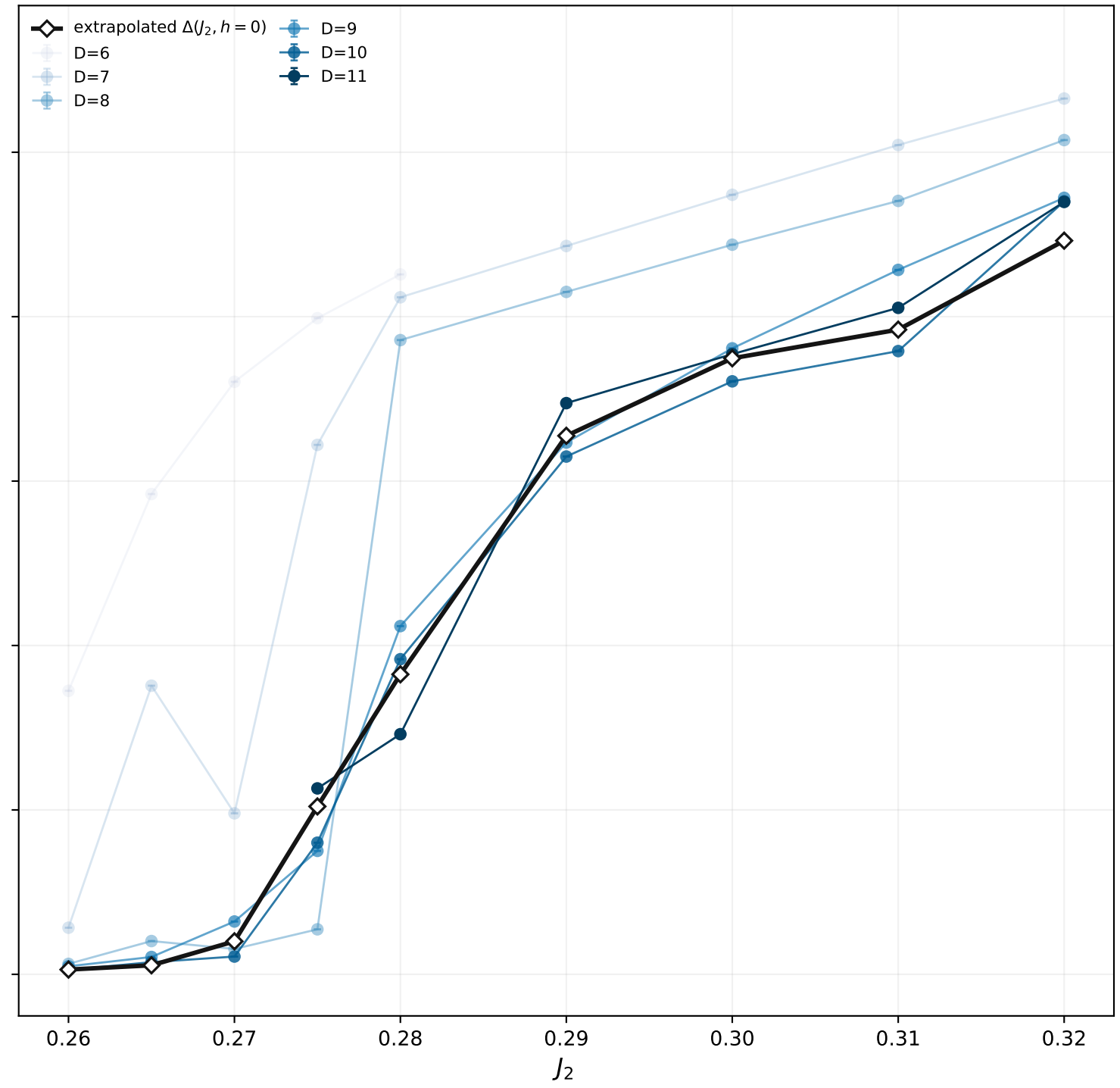
Plaquette sector
