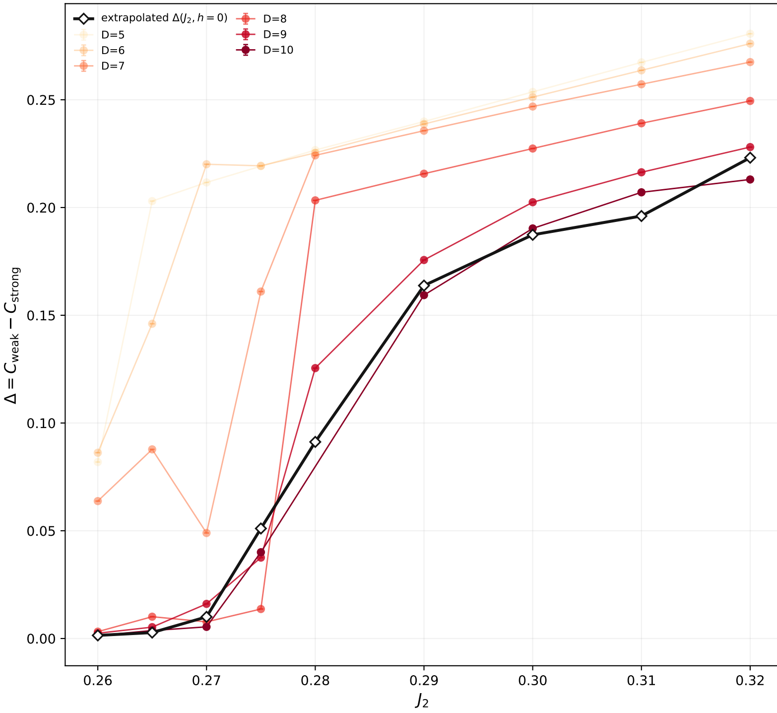
Dimer-plaquette sector
