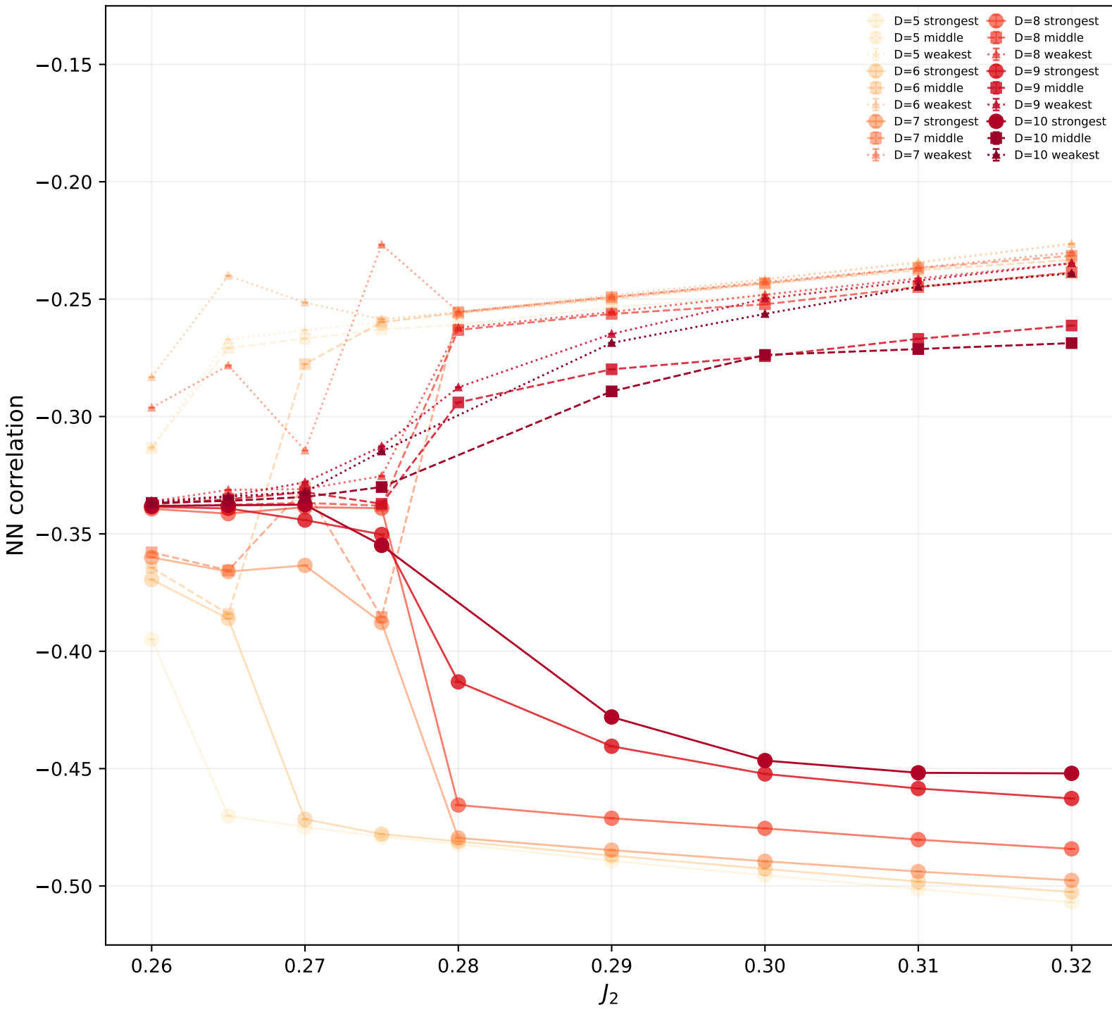
Dimer-plaquette sector
