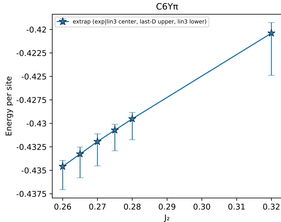
Energy per site vs J_2 — extrapolated
