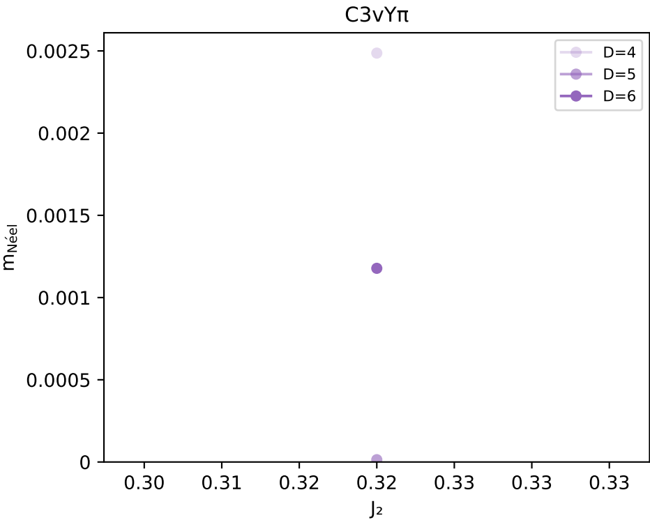
m_{\text{Néel}} vs J_2 — raw D curves
