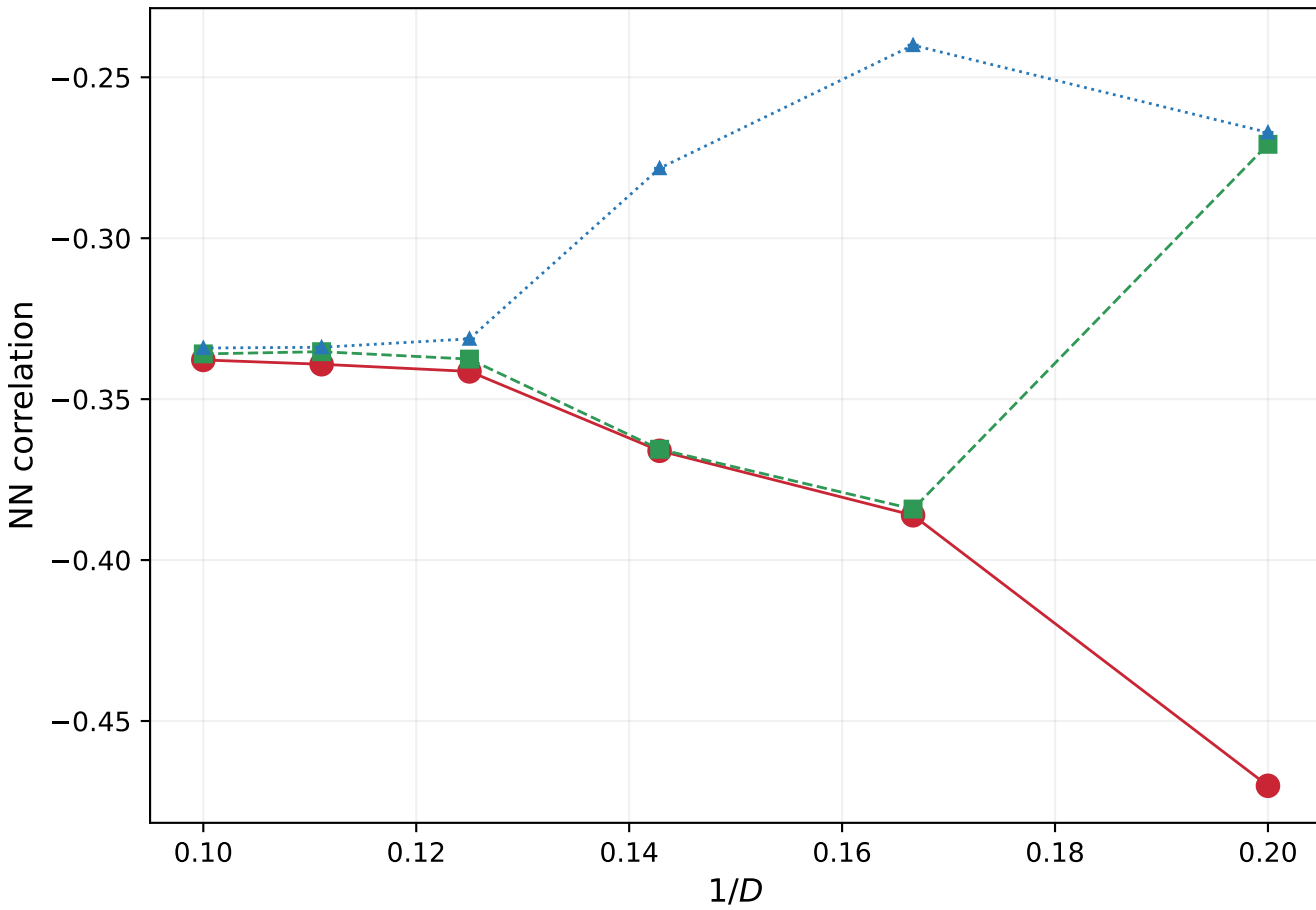
Dimer-plaquette sector, J_2 = 0.265
