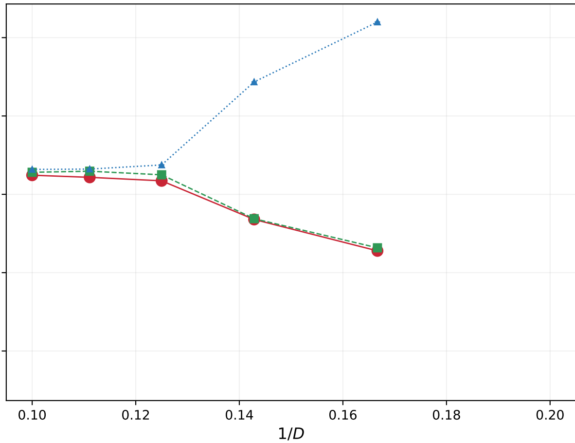
Plaquette sector, J_2 = 0.265
