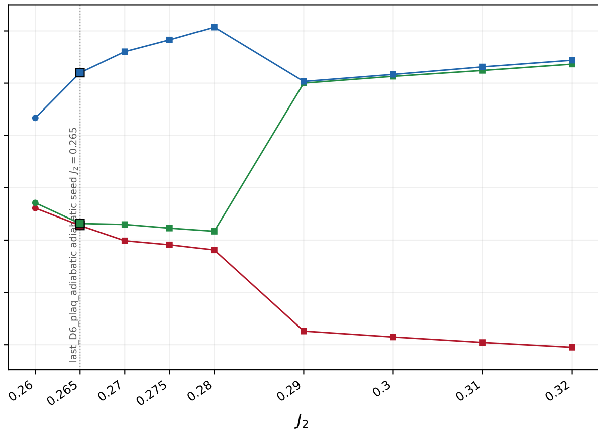
Plaquette sector, D = 6
