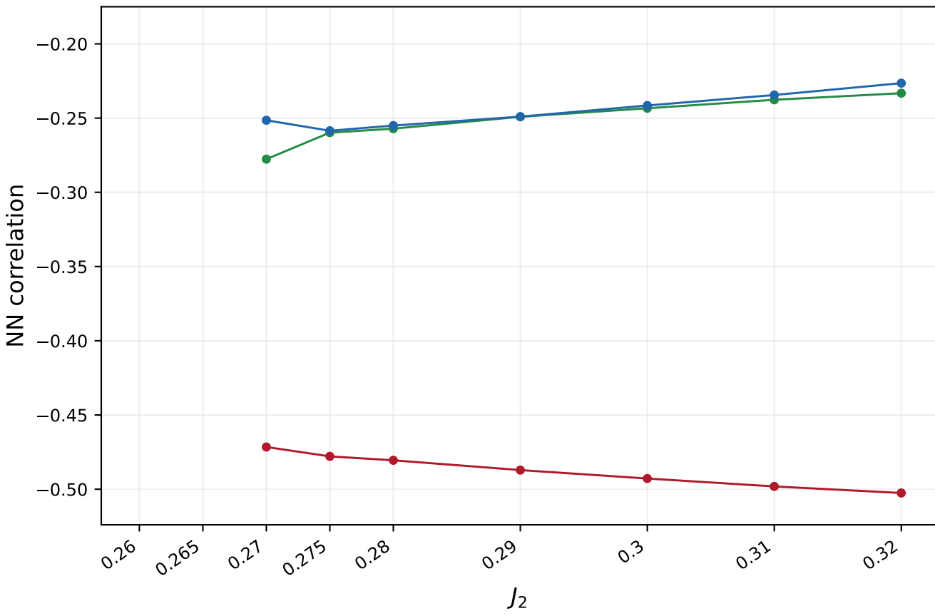
Dimer-plaquette sector, D = 6
