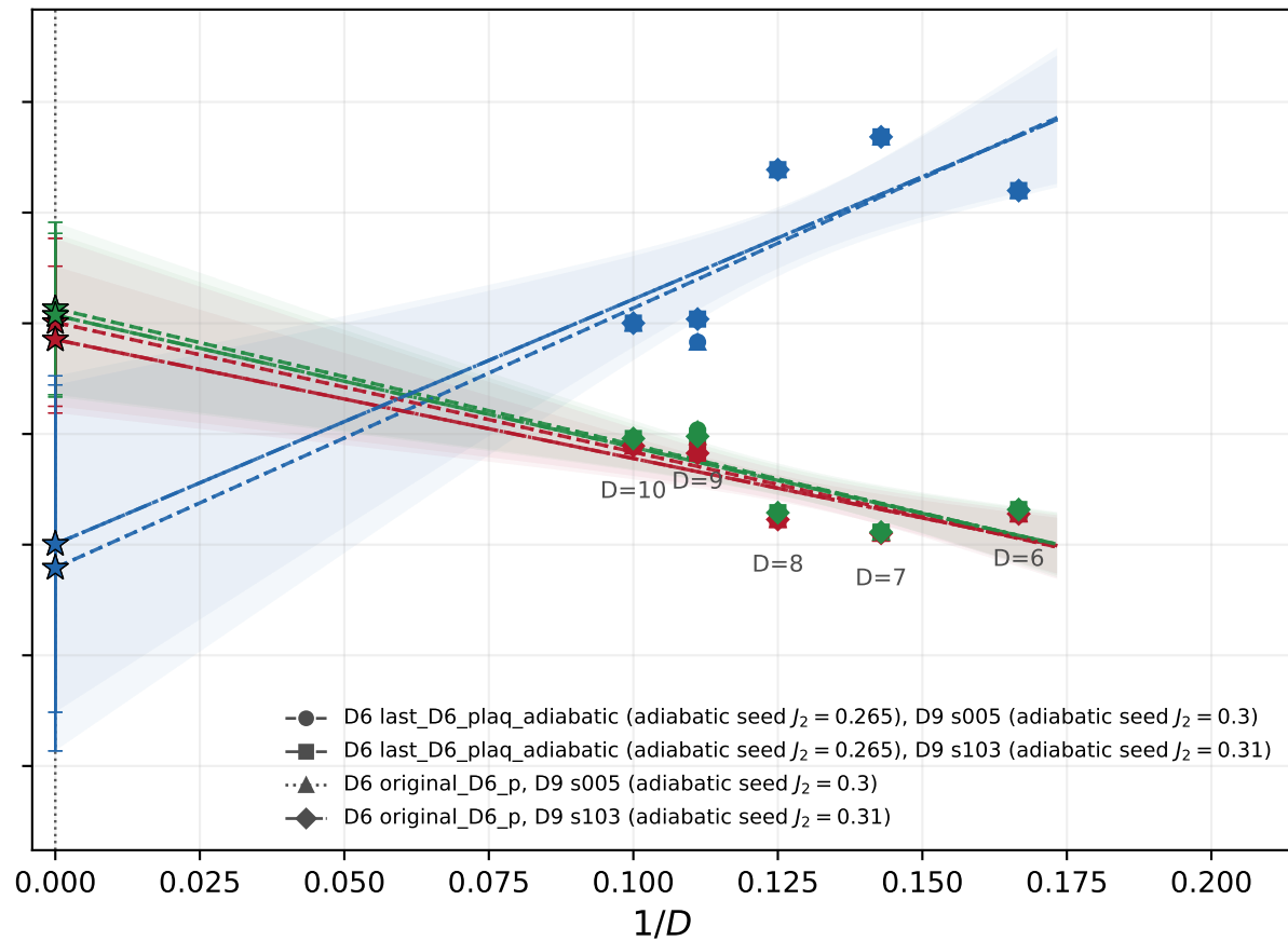
Plaquette sector, J_2 = 0.265
