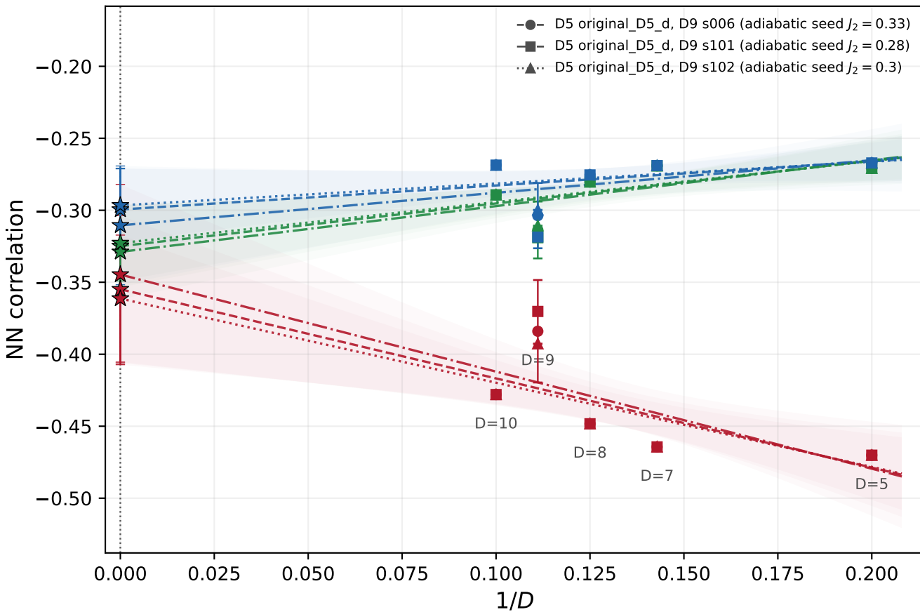
Dimer-plaquette sector, J_2 = 0.265
