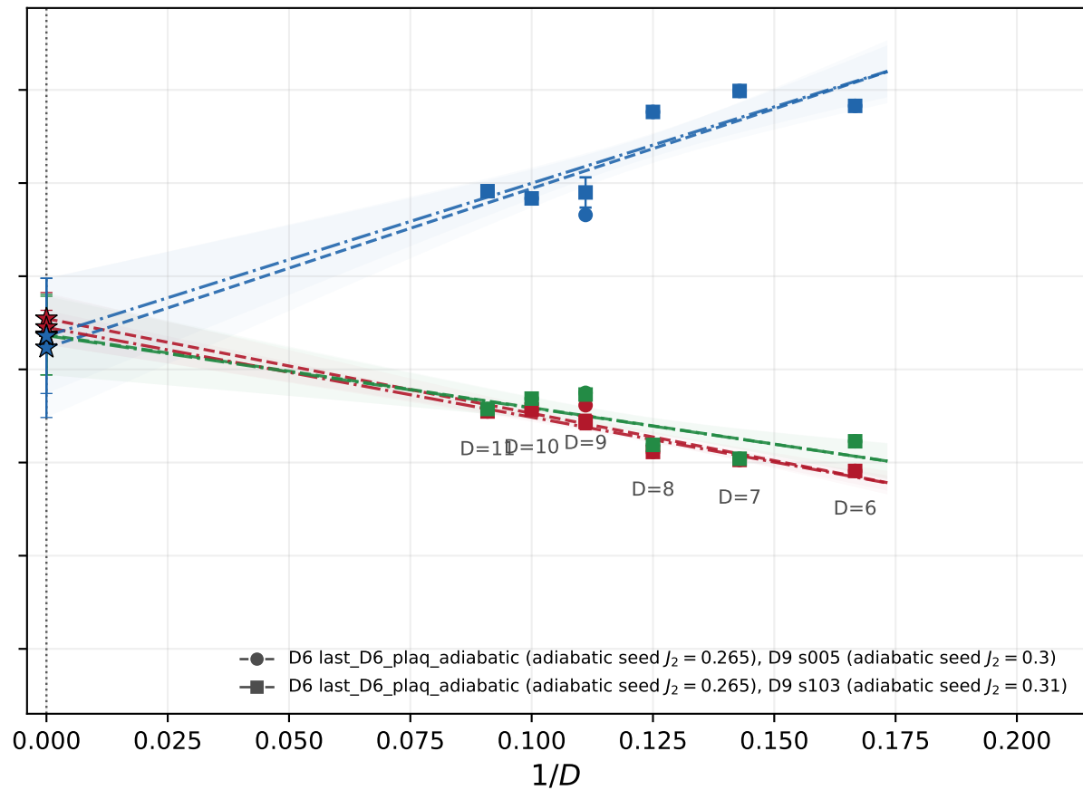
Plaquette sector, J_2 = 0.275
