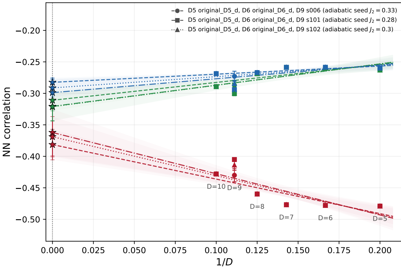
Dimer-plaquette sector, J_2 = 0.275
