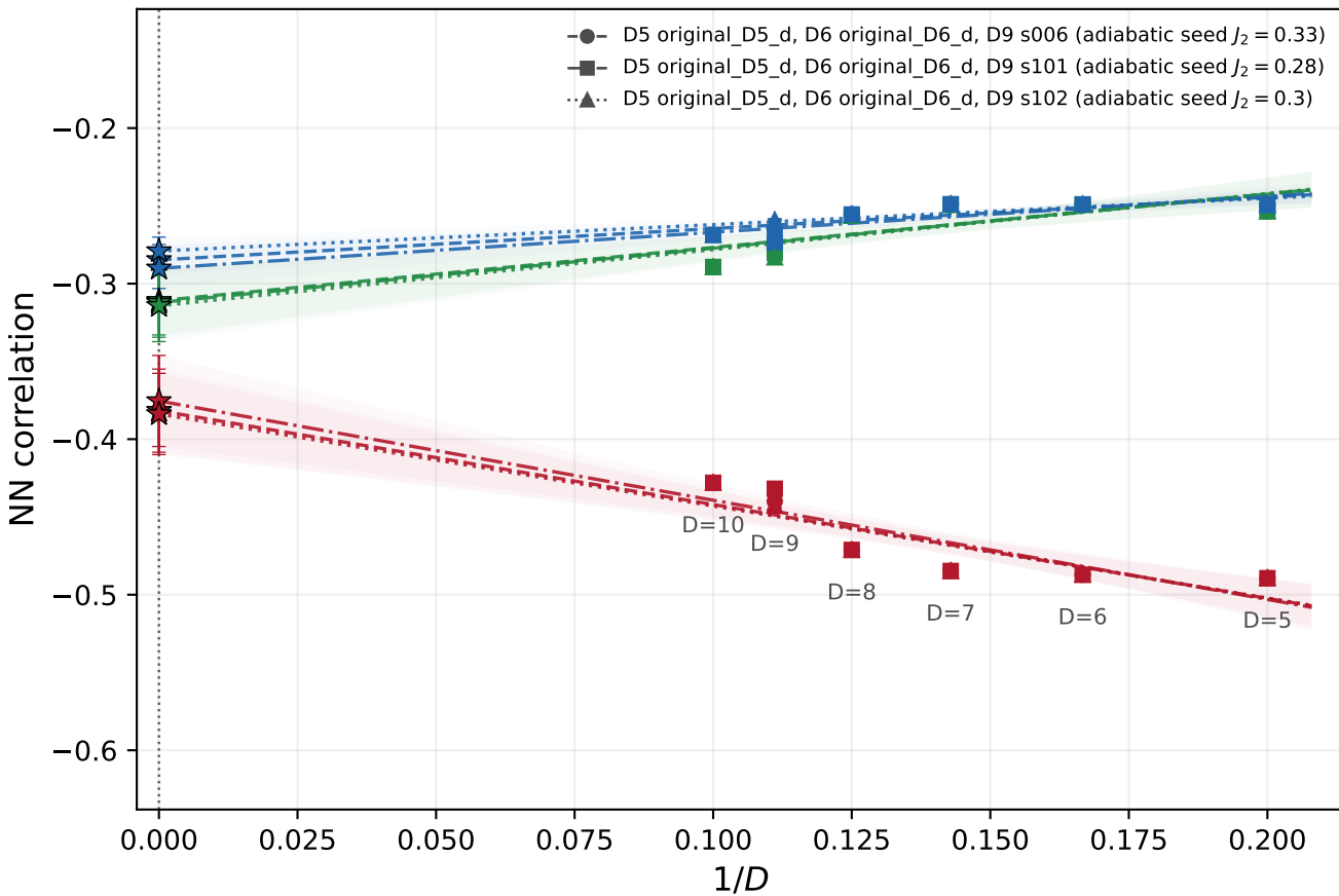
Dimer-plaquette sector, J_2 = 0.29
