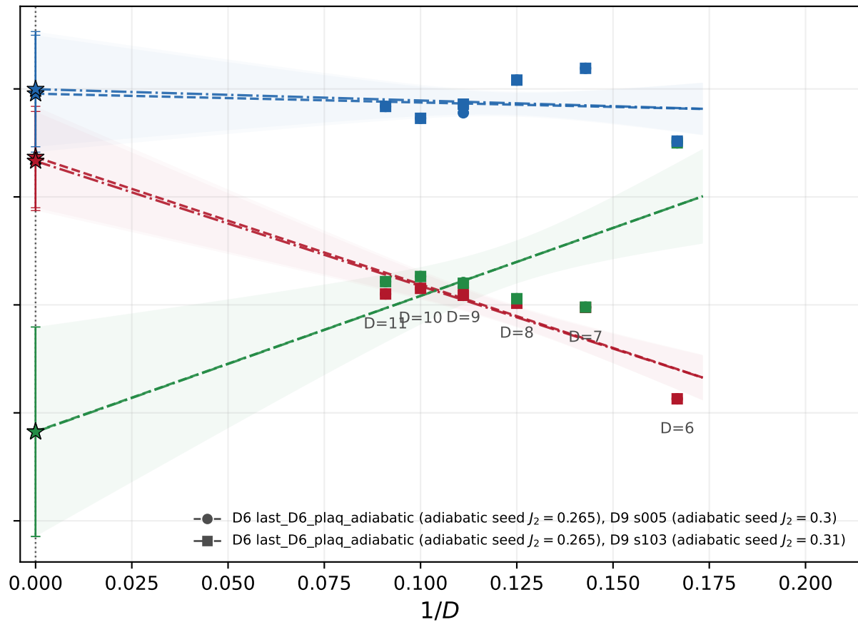
Plaquette sector, J_2 = 0.29
