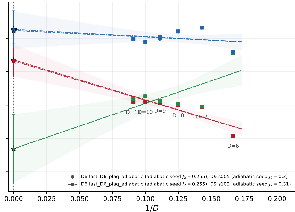
Plaquette sector, J_2 = 0.3
