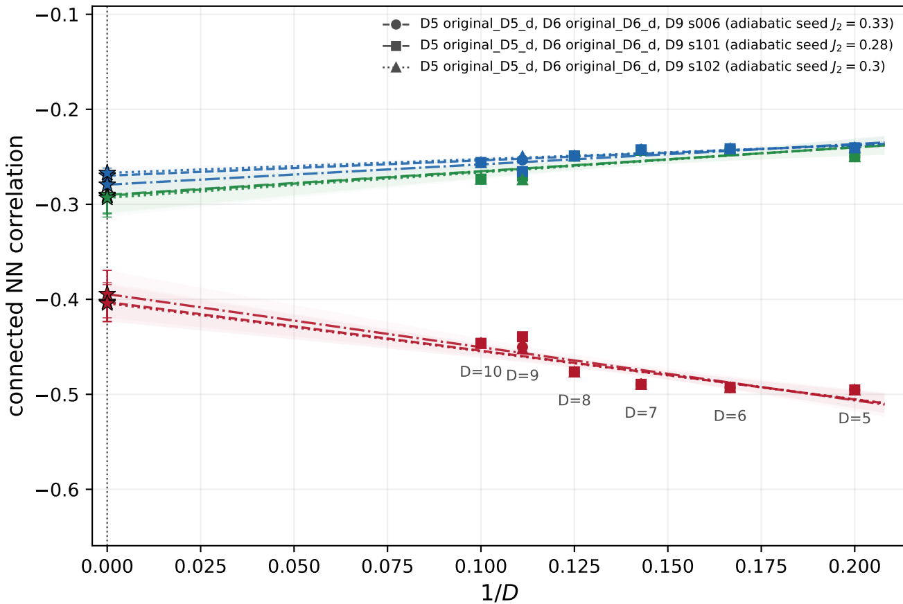
Dimer-plaquette sector, J_2 = 0.3
