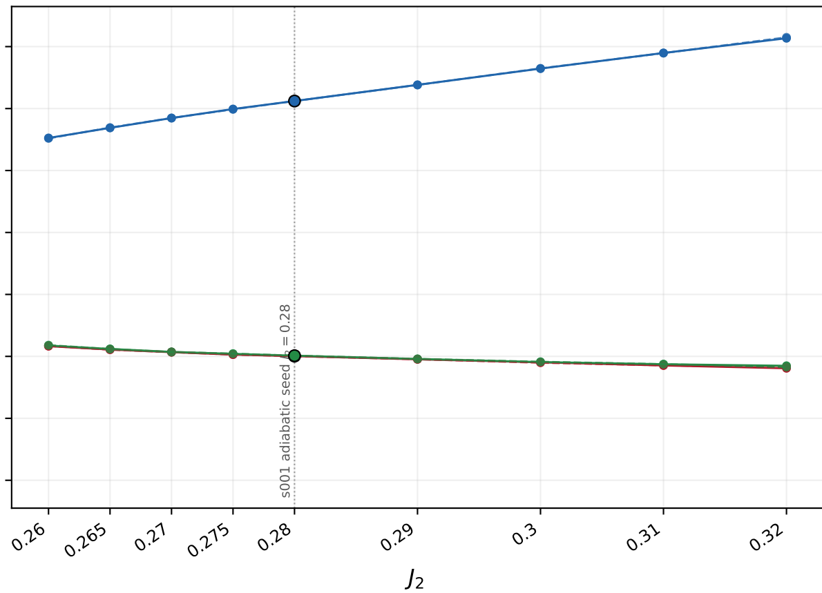
Plaquette sector, D = 7
