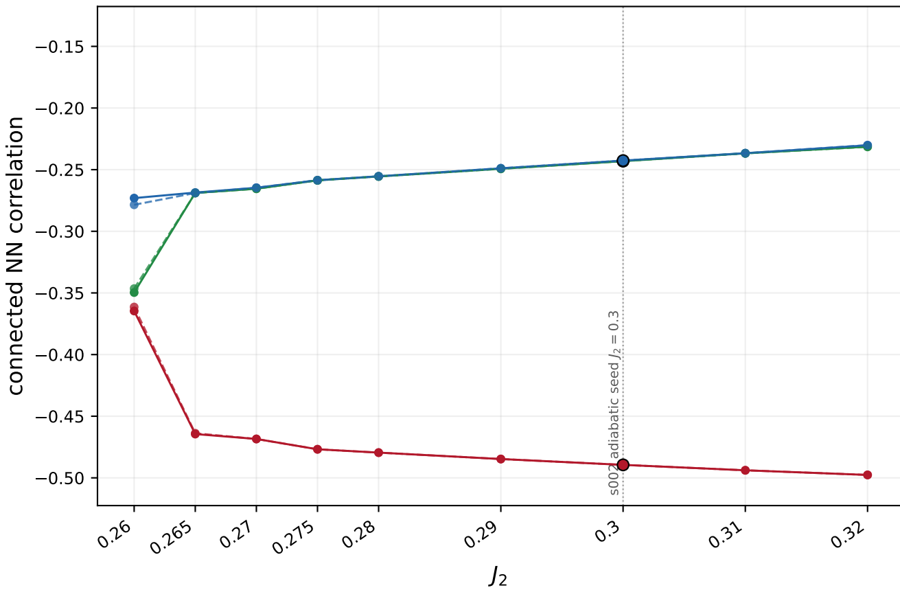
Dimer-plaquette sector, D = 7
