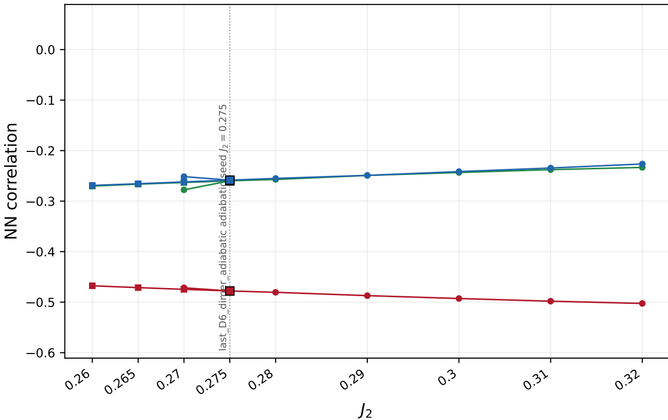
Dimer-plaquette sector, D = 6
