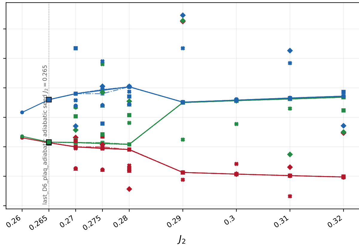
Plaquette sector, D = 6
