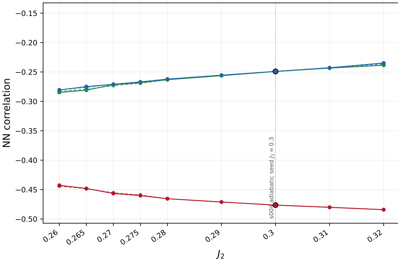
Dimer-plaquette sector, D = 8
