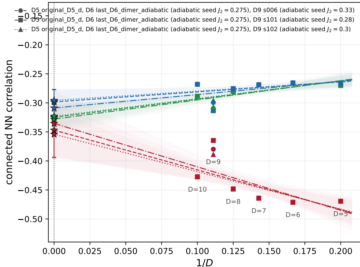
Dimer-plaquette sector, J_2 = 0.265
