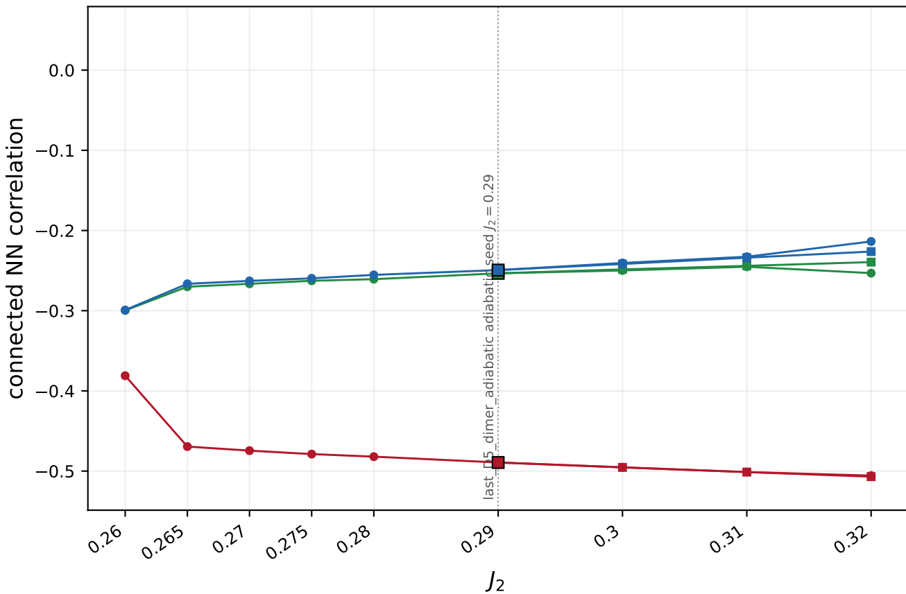
Dimer-plaquette sector, D = 5
