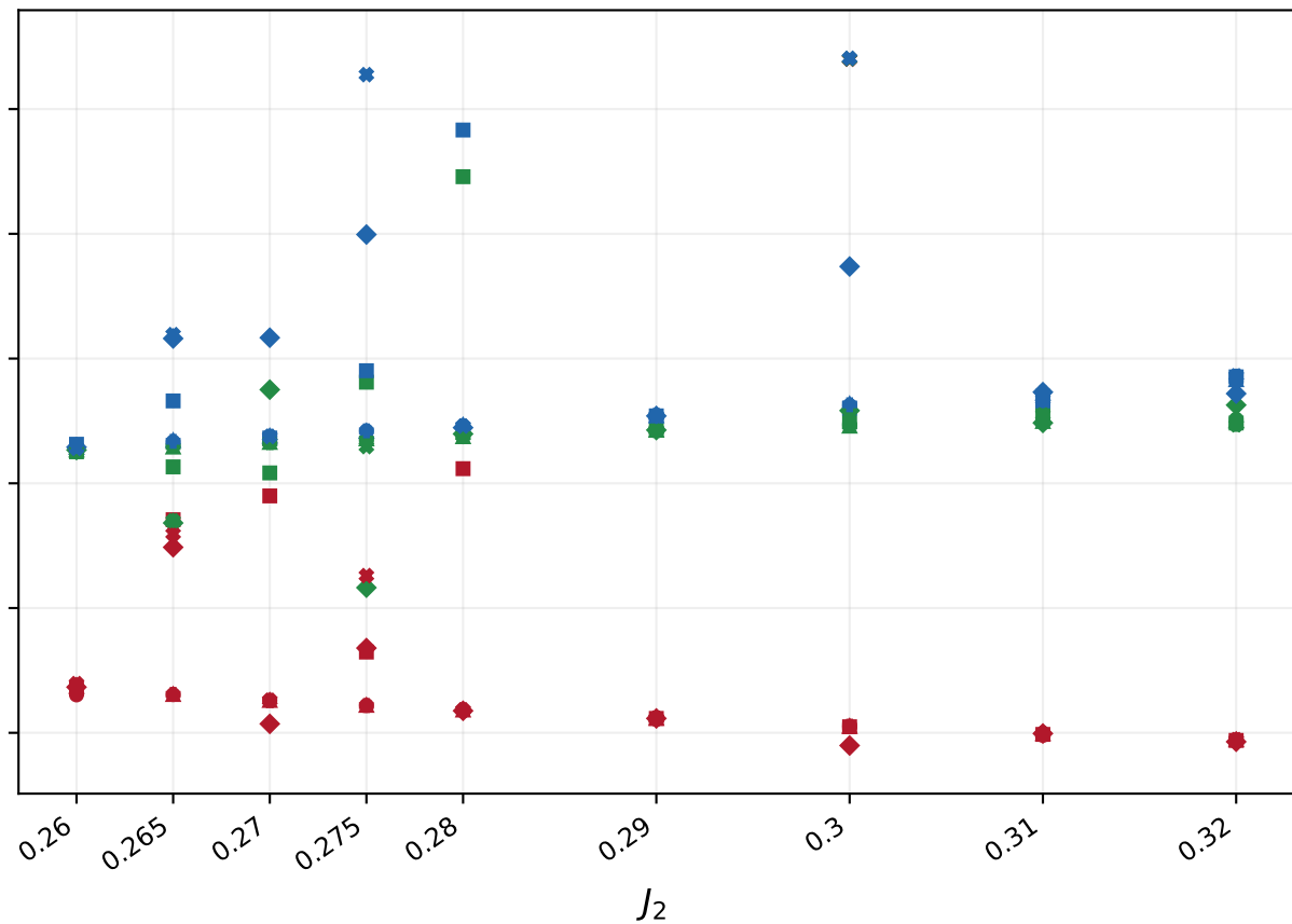
Plaquette sector, D = 5
