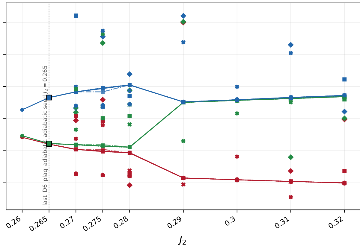
Plaquette sector, D = 6
